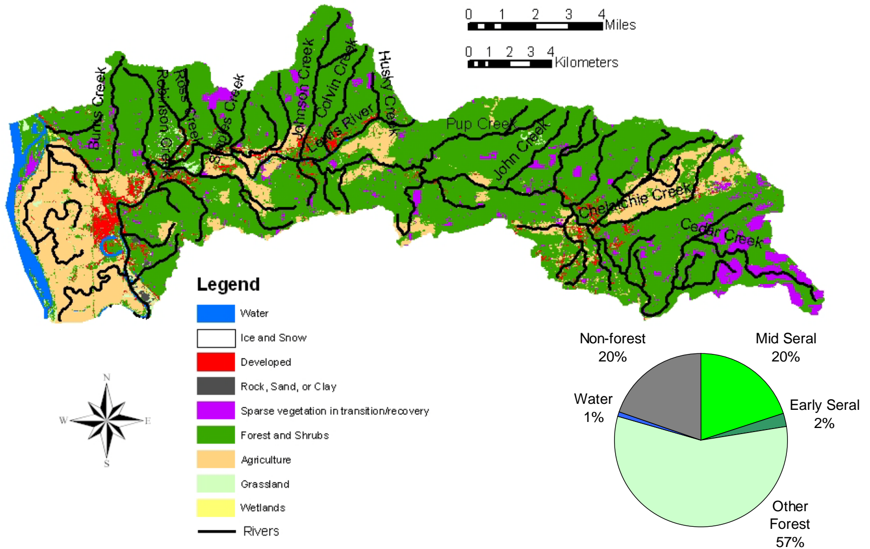
Figure K-3. Land cover within the lower North Fork Lewis River basin. Vegetation cover (pie chart) derived from Landsat data based on methods in Lunetta et al 1997. Data was obtained from the USGS National Land Cover Dataset (NLCD).
