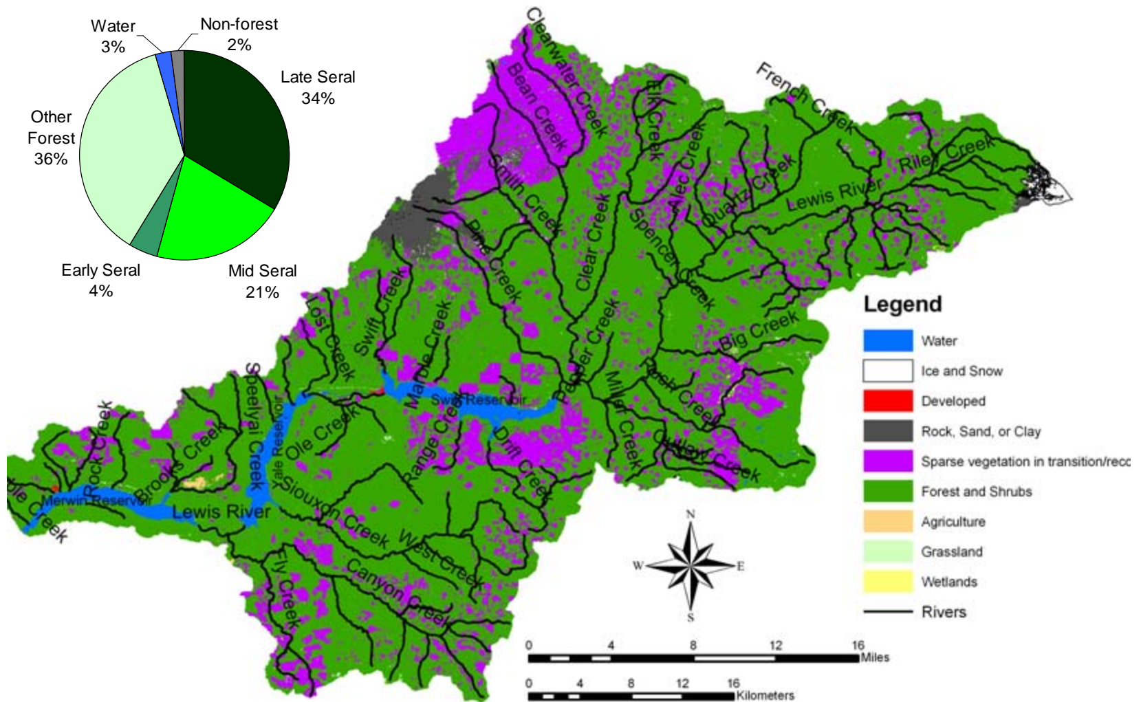
Figure K-24. Land cover within the upper North Fork Lewis basin. Vegetation cover (pie chart) derived from Landsat data based on methods in Lunetta et al. (1997). Mapped data was obtained from the USGS National Land Cover Dataset (NLCD).
