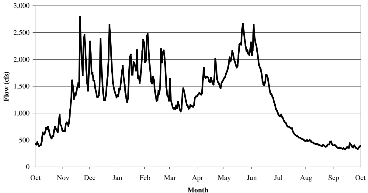
Figure K-25. Lewis River flow above reservoirs (Lewis River above Muddy Creek) for water years 1961-1970. These data exhibit the double humped hydrograph typical of a winter rain/rain-on-snow and spring snowmelt flow regime. USGS Gage #14216000; Lewis River above Muddy River near Cougar, Wash.
