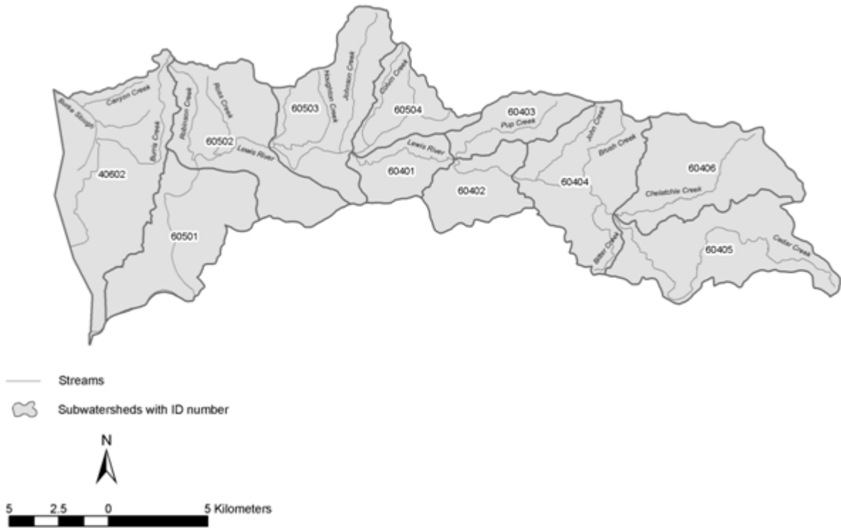
Figure K-15. Map of the Lower North Fork Lewis River basin showing the location of the IWA subwatersheds.
