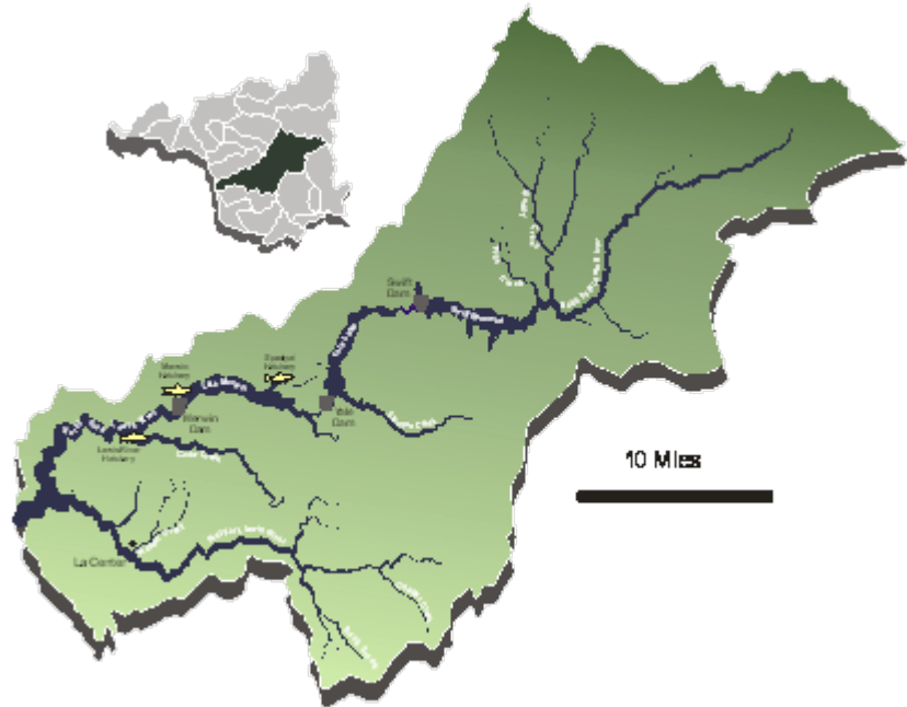
Figure K-22. Map of the North Fork Lewis River.
