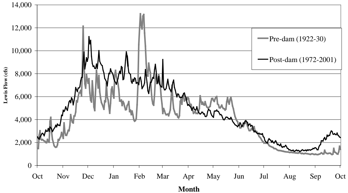
Figure K-4 Lower Lewis River flow pre- and post-Merwin Dam (1931). Hydro-regulation has decreased flows in the spring and increased flows in summer and fall. USGS Gage #14220500; Lewis River at Ariel, WA
