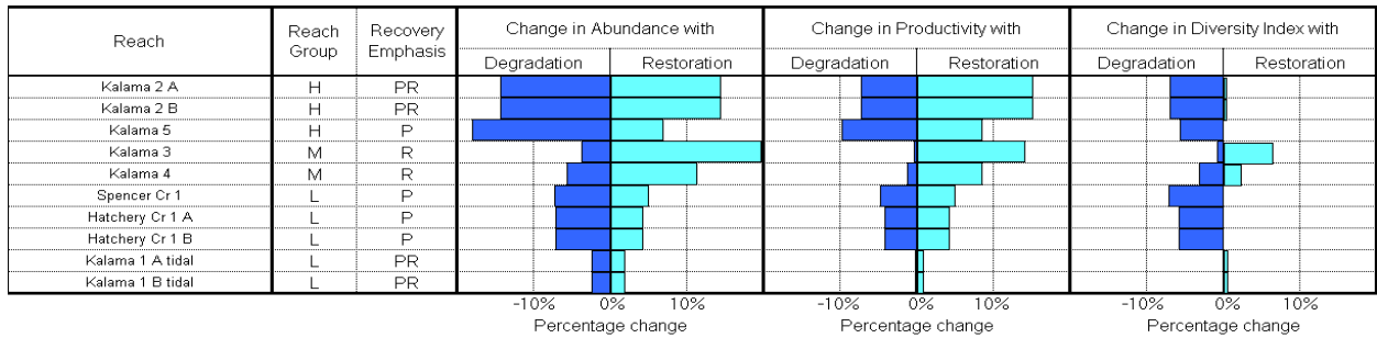
Figure J-10. Kalama subbasin chum ladder diagram. The rungs on the ladder represent the reaches and the three ladders contain a preservation value and restoration potential based on abundance, productivity, and diversity. The units in each rung are the percent change from the current population. For each reach, a reach group designation and recovery emphasis designation is given. Percentage change values are expressed as the change per 1000 meters of stream length within the reach. See Appendix E Chapter 6 for more information on EDT ladder diagrams. Some low priority reaches are not included for display purposes.
