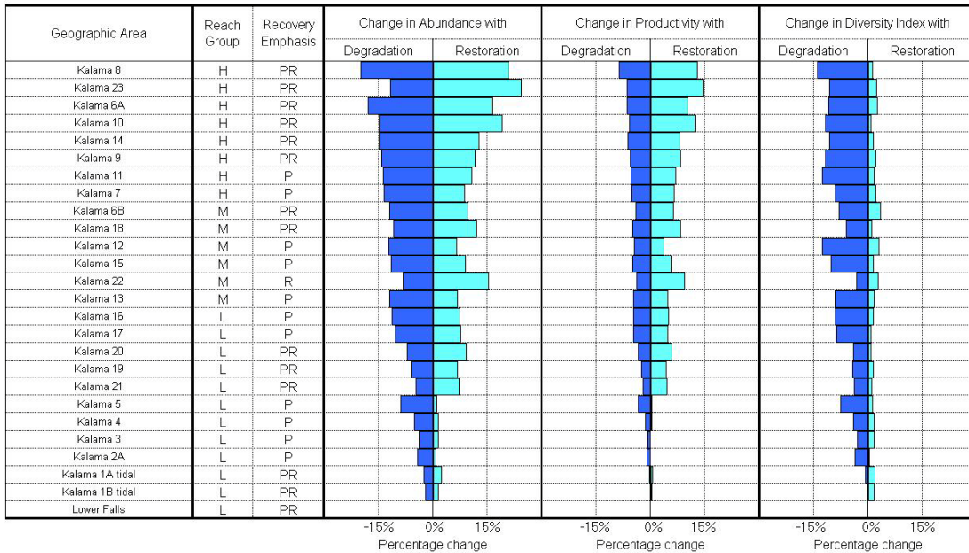
Figure J-12. Kalama subbasin spring Chinook ladder diagram. The rungs on the ladder represent the reaches and the three ladders contain a preservation value and restoration potential based on abundance, productivity, and diversity. The units in each rung are the percent change from the current population. For each reach, a reach group designation and recovery emphasis designation is given. Percentage change values are expressed as the change per 1000 meters of stream length within the reach. See Appendix E Chapter 6 for more information on EDT ladder diagrams. Some low priority reaches are not included for display purposes.
