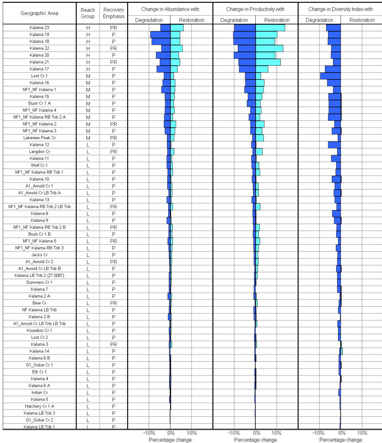
Figure J-7. Kalama River subbasin summer steelhead ladder diagram. The rungs on the ladder represent the reaches and the three ladders contain a preservation value and restoration potential based on abundance, productivity, and diversity. The units in each rung are the percent change from the current population. For each reach, a reach group designation and recovery emphasis designation is given. Percentage change values are expressed as the change per 1000 meters of stream length within the reach. See Appendix E Chapter 6 for more information on EDT ladder diagrams. Some low priority reaches are not included for display purposes.
