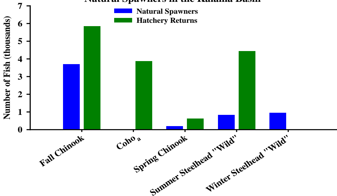
Figure J-22. Recent average hatchery returns and estimates of natural spawning escapement in the Kalama River basins by species. The years used to calculate averages varied by species, based on available data. The data used to calculate average hatchery returns and natural escapement for a particular species and basin were derived from the same years in all cases. All data were from the period 1992 to the present, except for Kalama wild summer steelhead, which represents the 1988–99 average. Calculation of each average utilized a minimum of 5 years of data, except for Kalama wild winter steelhead, which only includes 2000 escapement data.
