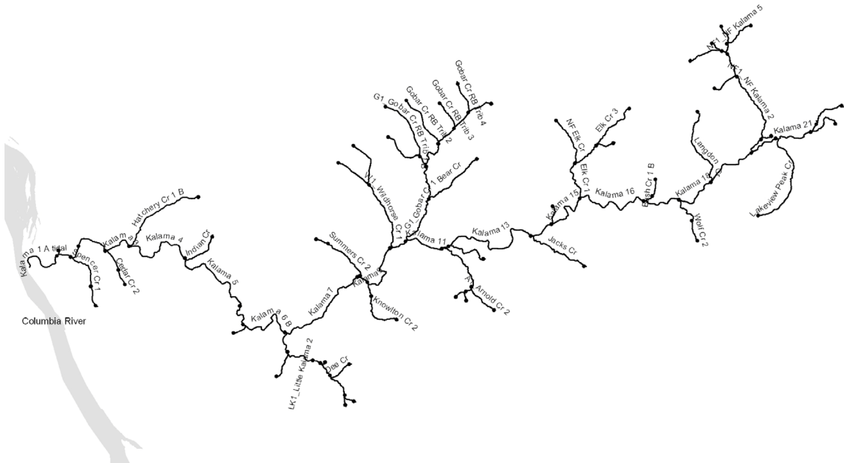
Figure J-6. Kalama Subbasin with EDT reaches identified. For readability, not all reaches are labeled.
