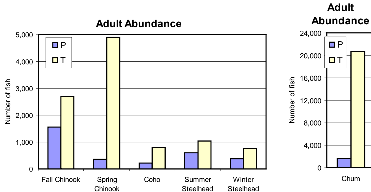
Figure J-5. Adult abundance of Kalama fall Chinook, spring Chinook, coho, winter steelhead, summer steelhead and chum based on EDT analysis of current (P or patient) and historical (T or template) habitat conditions.
