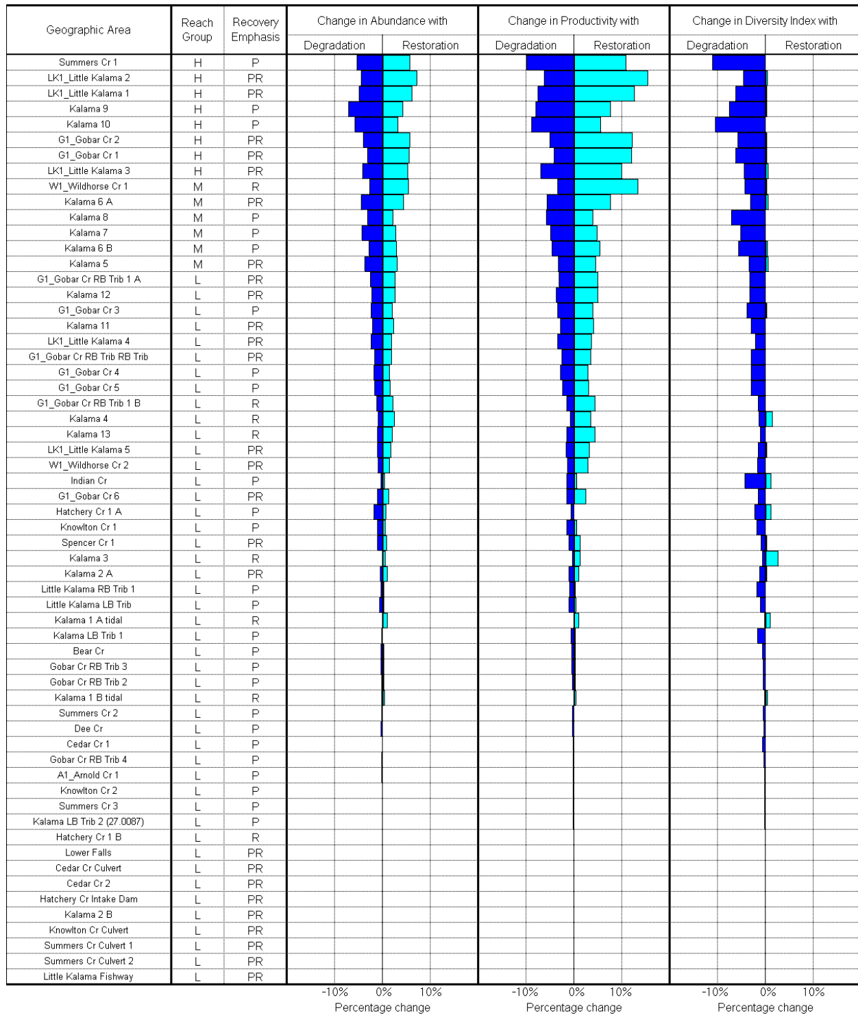
Figure J-8. Kalama subbasin winter steelhead ladder diagram. The rungs on the ladder represent the reaches and the three ladders contain a preservation value and restoration potential based on abundance, productivity, and diversity. The units in each rung are the percent change from the current population. For each reach, a reach group designation and recovery emphasis designation is given. Percentage change values are expressed as the change per 1000 meters of stream length within the reach. See Appendix E Chapter 6 for more information on EDT ladder diagrams. Some low priority reaches are not included for display purposes.
