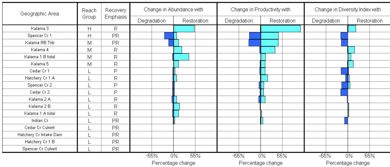
Figure J-11. Kalama subbasin coho ladder diagram. The rungs on the ladder represent the reaches and the three ladders contain a preservation value and restoration potential based on abundance, productivity, and diversity. The units in each rung are the percent change from the current population. For each reach, a reach group designation and recovery emphasis designation is given. Percentage change values are expressed as the change per 1000 meters of stream length within the reach. See Appendix E Chapter 6 for more information on EDT ladder diagrams. Some low priority reaches are not included for display purposes.
