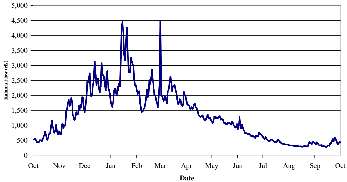
Figure J-4. Kalama River hydrograph (1966-1975). Values are daily mean flows. The Kalama exhibits a fall through spring rainfall dominated regime, with flows typically falling below 300 cfs in late summer. Data is from USGS Stream Gage #14223500; Kalama River below Italian Cr. near Kalama, WA.
