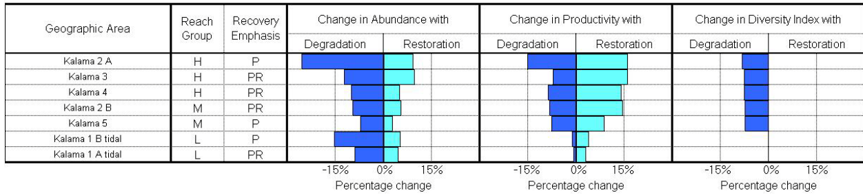
Figure J-9. Kalama subbasin fall Chinook ladder diagram. The rungs on the ladder represent the reaches and the three ladders contain a preservation value and restoration potential based on abundance, productivity, and diversity. The units in each rung are the percent change from the current population. For each reach, a reach group designation and recovery emphasis designation is given. Percentage change values are expressed as the change per 1000 meters of stream length within the reach. See Appendix E Chapter 6 for more information on EDT ladder diagrams. Some low priority reaches are not included for display purposes.
