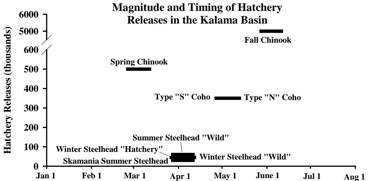
Figure J-21. Magnitude and timing of hatchery releases in the Kalama River basin by species, based on 2003 brood production goals.
