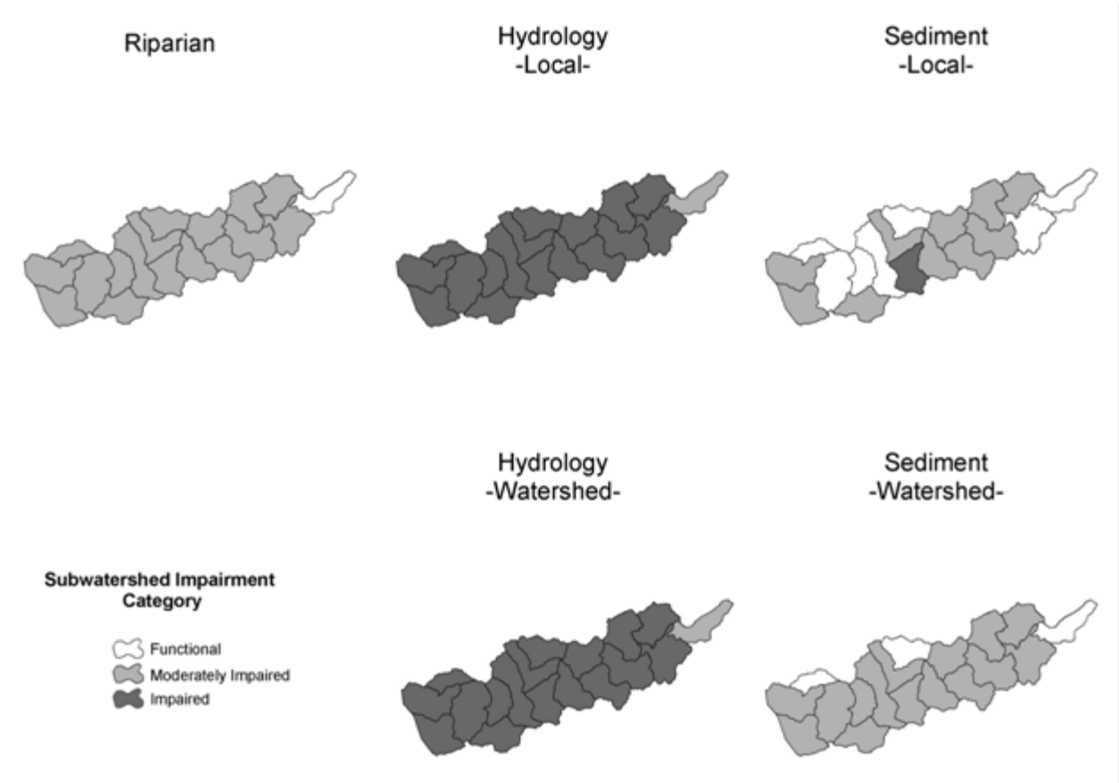
Figure J-20. IWA subwatershed impairment ratings by category for the Kalama Subbasin
