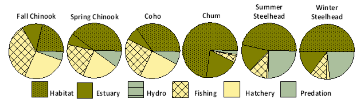
Figure J-23. Relative contribution of potentially manageable impacts on Kalama River salmonid populations.
